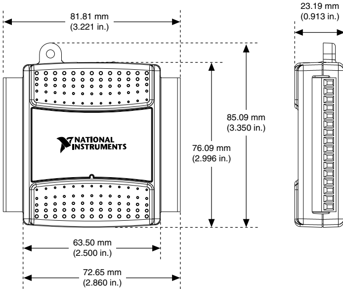
Figure 1. USB-6008 Dimensions
