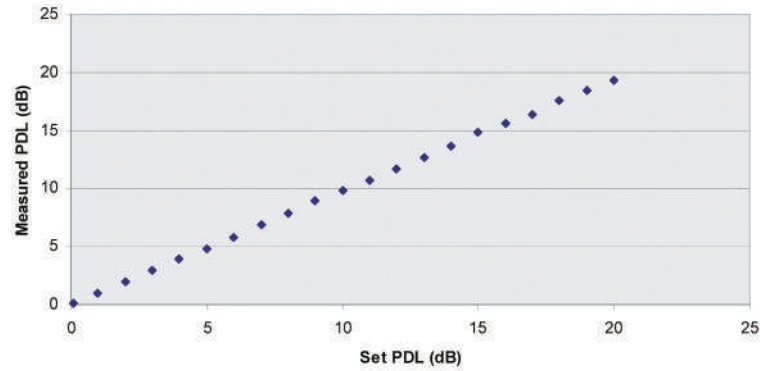
Figure 1. PDL generation accuracy: PDL generated by the PDLE-101 PDL Source/Emulator, measured using a PDL-101 PDL meter.
