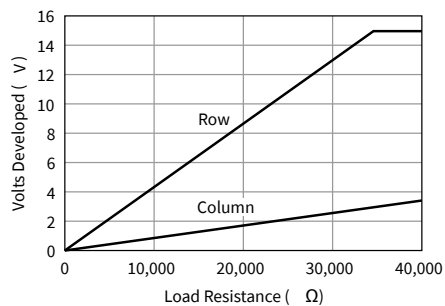
Figure 1. Impact of Charge Injection at Power Up: Typical Voltage Developed vs. Resistive Load (Using Test Setup in Figure 2)
