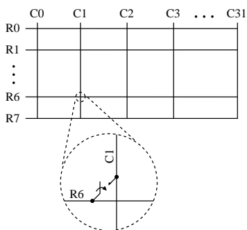
Figure 1. NI 2534 Hardware Diagram
