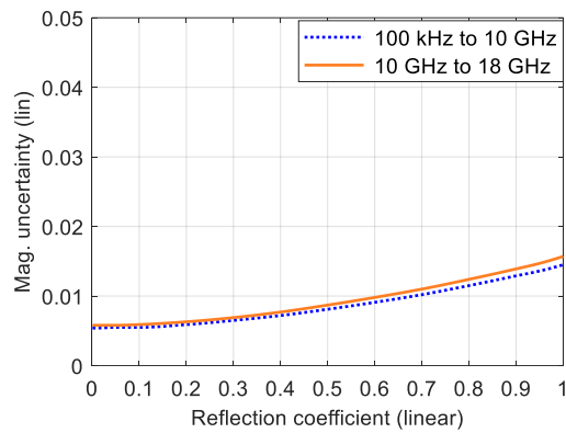
Measured uncertainty of reflection magnitude and reflection phase measurements for the R&S®ZNLE 1 ; analysis conditions: S_{12} = S_{21} = 0 , calibrated power -10 dBm, measured power -10 dBm
