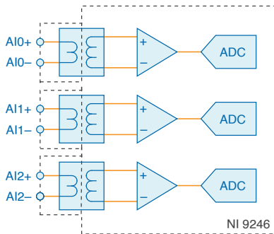
Figure 1. NI 9246 Input Circuitry
