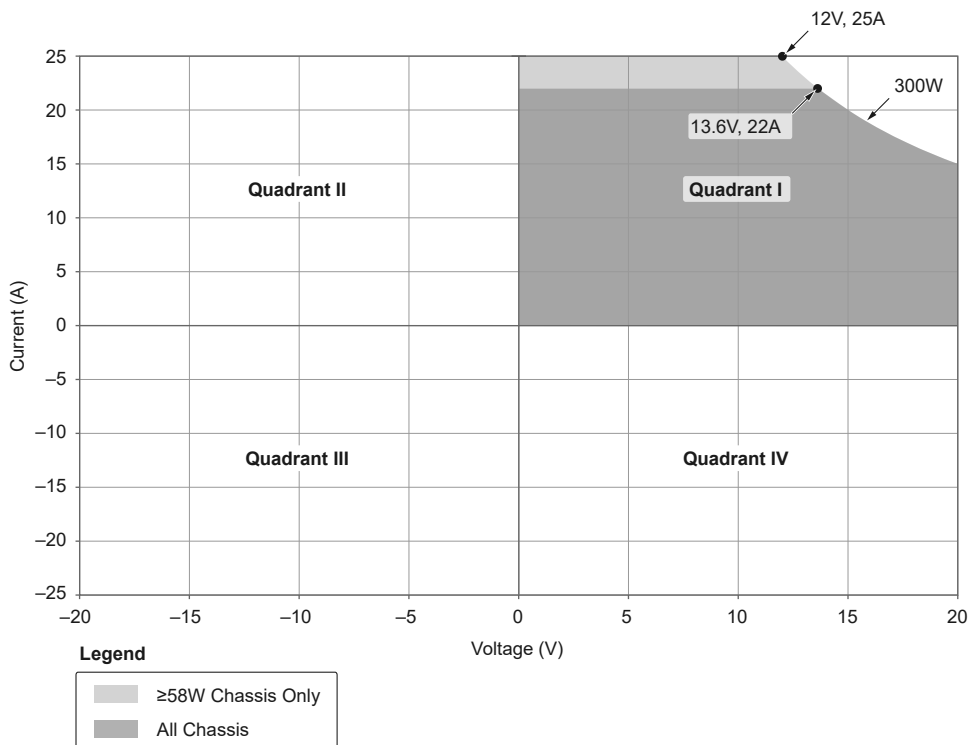
Figure 1. PXIe-4151 Quadrant Diagram, T_{\text{ambient}} = 0\text{ }^{\circ}\text{C} to 40\text{ }^{\circ}\text{C}
