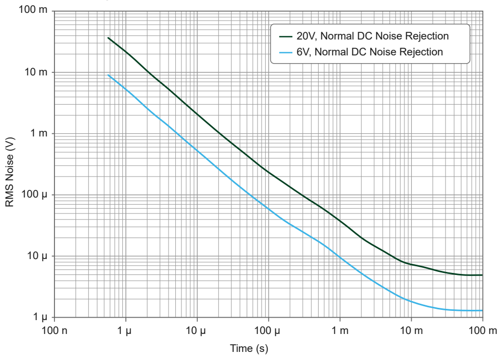
Figure 3. Voltage RMS Noise Versus Aperture Time, Nominal
