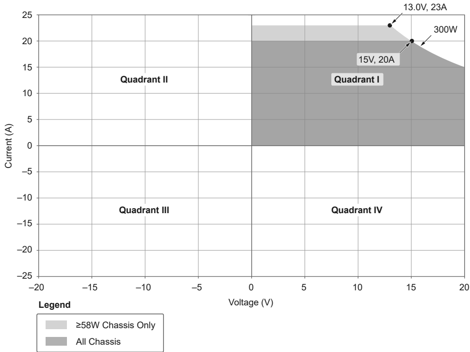
Figure 2. PXIe-4151 Quadrant Diagram, T_{\text{ambient}} > 40\text{ }^{\circ}\text{C}
