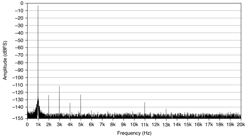
Figure 10. -3 dBFS, 1 kHz Tone Acquired at 1.25 MSample/s, 1 V Range (Full Bandwidth)
