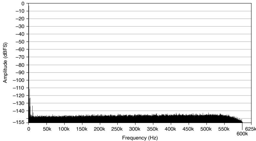
Figure 8. -3 dBFS, 1 kHz Tone Acquired at 1.25 MSample/s, 5 V Range (Full Bandwidth)
