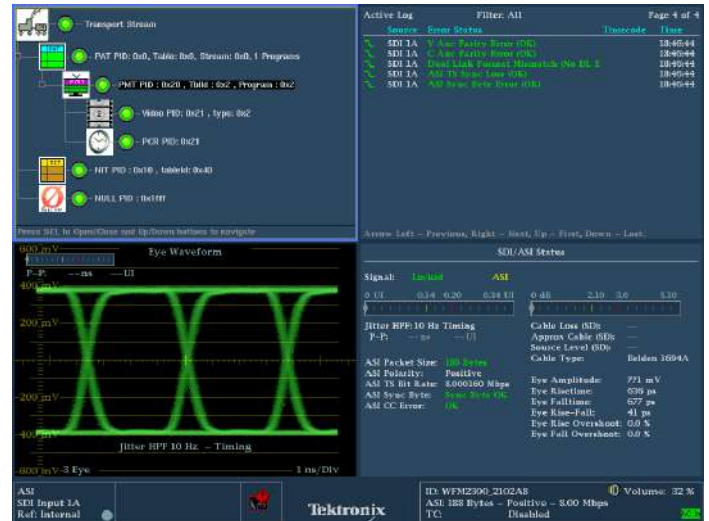
ASI monitoring (MPEG2 PID Tree display, Error Log status display, Eye pattern measurement display, SDI/ASI Status display) is available with Option ASI.
