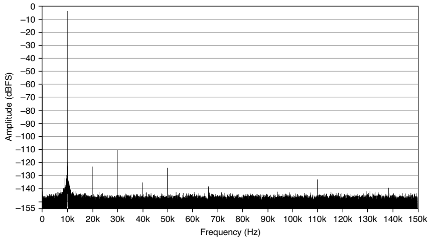
Figure 18. -3 dBFS, 10 kHz Tone Acquired at 1.25 MSample/s, 0.5 V Range (Full Bandwidth)
