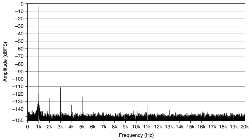
Figure 10. -3 dBFS, 1 kHz Tone Acquired at 1.25 MSample/s, 0.5 V Range (Full Bandwidth)
